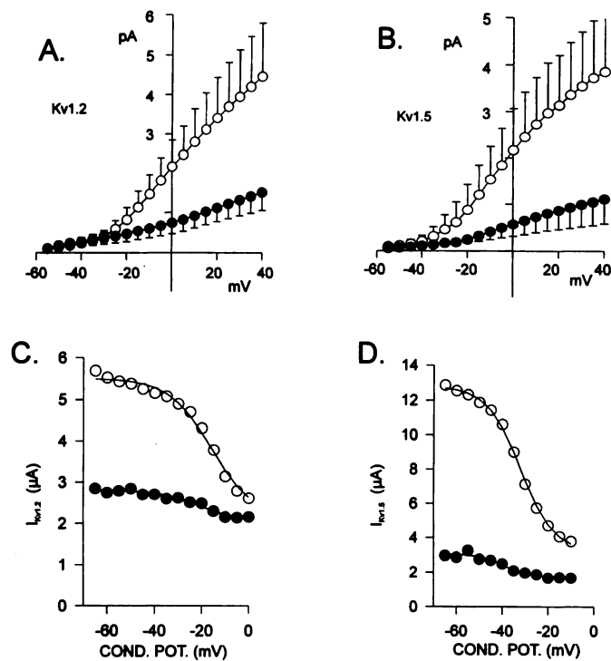
Fig. 2. Effect of ACh on I-V relationships and steady state inactivation of I_{Kv1.2} and I_{Kv1.5} . A, I-V relationship for I_{Kv1.2} before (○) and 20 min after (●) application of ACh 100 \mu M (five). B, I-V relationship for I_{Kv1.5} before (○) and 20 min after (●) application of ACh 100 \mu M (eight). C, Steady state inactivation of I_{Kv1.2} (control, ○; ACh, ●). V_{0.5} was shifted negative by ACh from -16 to -21 mV (two). D, Steady state inactivation of I_{Kv1.5} (control, ○; ACh, ●). V_{0.5} was also shifted negative by ACh from -32 to -39 mV (two). Steady state inactivation was studied using 15-sec conditioning steps to potentials ranging from -70 to +20 mV, followed by a 200-msec test pulse to +40 mV. The test currents elicited by the pulses to +40 mV were averaged and plotted as a function of conditioning potential. The data points were fitted with a Boltzmann function: G = (I_{test} - C)/(1 + \exp[(V - V_{0.5})/V_s]) + C , where I_{test} is the peak current elicited by the test pulse, V is the conditioning voltage, V_{0.5} is the voltage of half-maximal inactivation, V_s is the slope factor, and C is the magnitude of the noninactivating current component.
