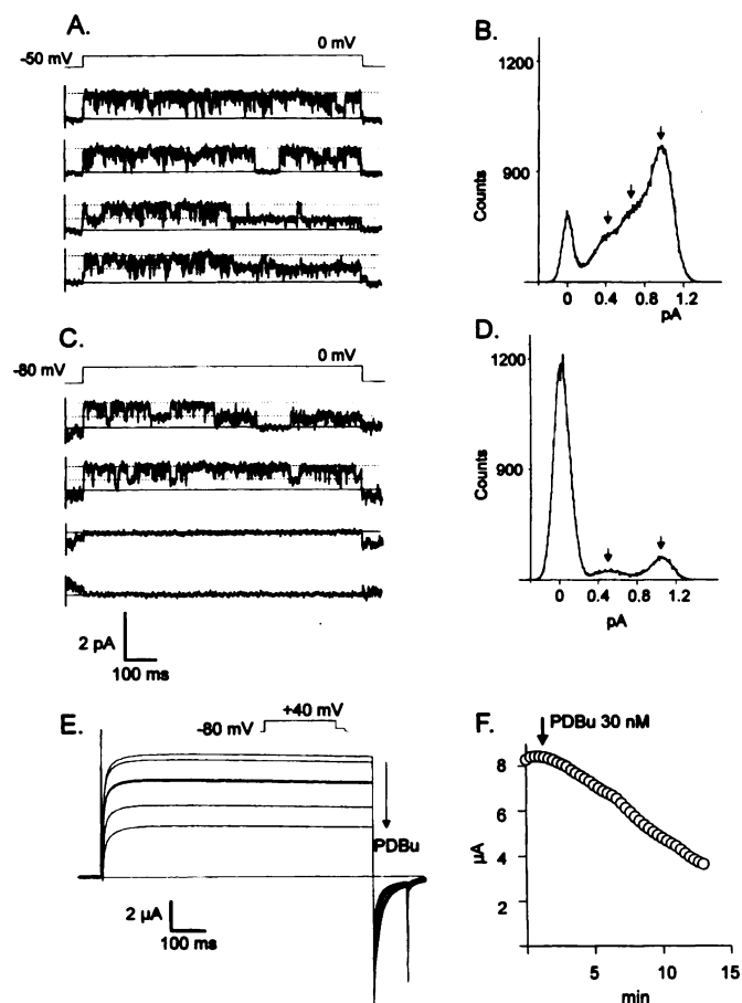
Fig. 6. Extra-patch application of PDBu decreases the open probability of K_v1.2 channels. A, Cell-attached recording as in Fig. 4A. Unitary channel openings were elicited by adjusting the holding potential ( V_h ) to -50 mV and applying depolarizing steps to 0 mV every 8 sec. B, All-points histogram of events at 0 mV. Note multiple subconductance states in this channel. NP_o = 0.892 . C, At 20 min after application of PDBu 30 nM to the cell membrane outside the patch, depolarization of the patch to 0 mV elicited no openings. However, some channel openings could be elicited by increasing V_h to -80 mV. The majority of the 20 episodes contained no channel openings. D, All-point histogram of the events at 0 mV in the presence of PDBu from V_h = -80 mV. Fully open channel current was unaffected but NP_o was markedly reduced to 0.185 . E, Whole-oocyte currents evoked during application of PDBu. Test depolarization to +40 mV. F, Time course of decrease of I_{Kv1.2} on application of PDBu 30 nM (arrow). This effect was not readily reversible.
