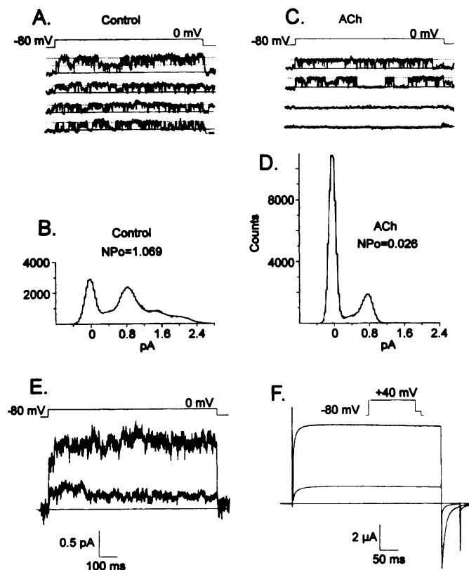
Fig. 5. Muscarinic ( m_3 ) receptor stimulation decreases the open probability of K_v1.2 channels via a diffusible intracellular second messenger. The oocyte was coinjected with hm_3 and K_v1.2 cRNAs. A, Cell-attached patch recording. Oocyte was bathed in high- K^+ solution (140 mM). Pipette solution contained 2 mM K^+ . The patch was depolarized from a holding potential of -80 mV to a test potential of 0 mV for 900 msec every 8 sec, which evoked opening of K_v1.2 channels after a short latency. At least two channels are evident in this patch. B, All-points histograms constructed from the channel activity recorded at 0 mV. Unitary current was estimated as 0.8 pA, and NP_o was estimated from the areas under the fitted gaussian curves as 1.069 . C, 20 min after application of ACh 100 \mu M to the membrane outside the patch, depolarization to 0 mV elicited fewer channel openings. Four episodes containing channel openings are shown. The majority of the 20 episodes contained no channel openings. D, All-points histogram of events at 0 mV after application of ACh. Note that unitary current is unchanged, but NP_o was decreased to 0.026 . E, Ensemble averaged currents from 20 consecutive episodes as depicted in A and C, before and after application of ACh. F, Whole-oocyte currents recorded from the same oocyte before and 16 min after application of ACh. Test potential, +40 mV. Note parallel reduction in whole-oocyte current and ensemble averaged patch current shown in E.
