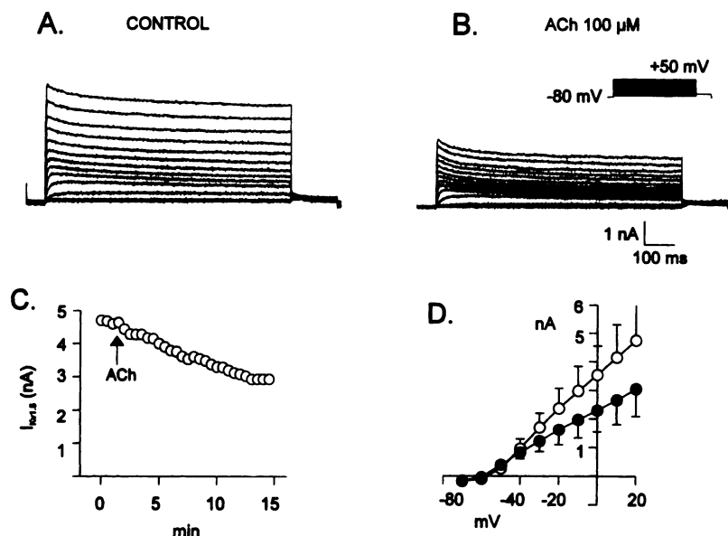
Fig. 8. Effect of ACh on whole-cell I_{Kv1.5} recorded from stably transfected COS cells cotransfected with hm3 receptor. A , Control currents. Cell was depolarized from a holding potential of -80 mV to test potentials ranging from -70 to +50 mV in 10 -mV increments every 8 sec. B , Currents elicited in the same cell in response to the same stimuli as in A after the application of ACh ( 100 \mu M). C , Time course of suppression of I_{Kv1.5} in response to ACh application (arrow). D , Mean I - V relationship of I_{Kv1.5} before ( \circ ) and after ( \bullet ) application of ACh (four).
